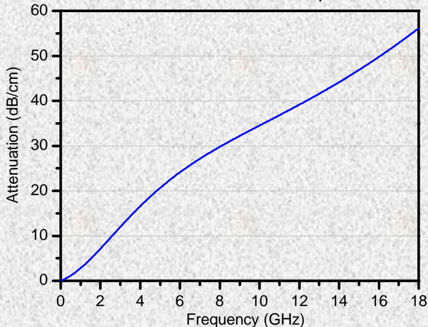
Attenuation of OP-7500 Spec01
