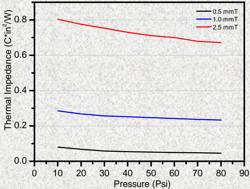
Thermal Impedance of OP-7500 Spec 01
