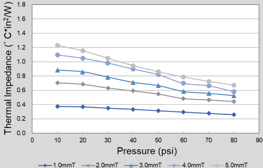
Thermal Impedance of OP-8500 Spec07
