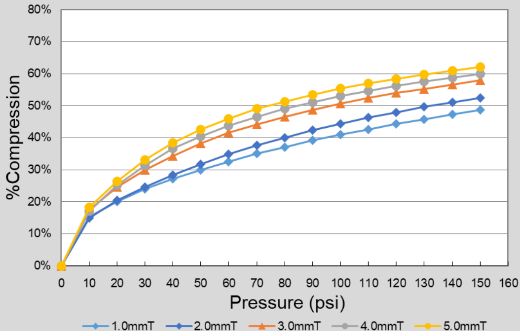
% Compression of OP-8500 Spec07
