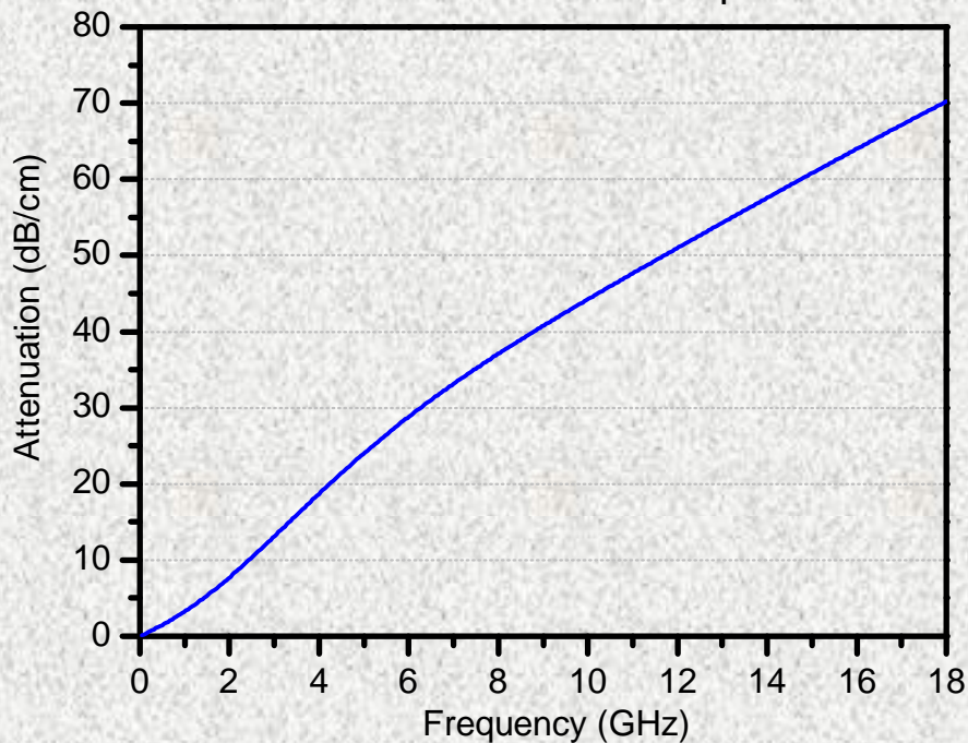
Attenuation of OP-7600 Spec01
