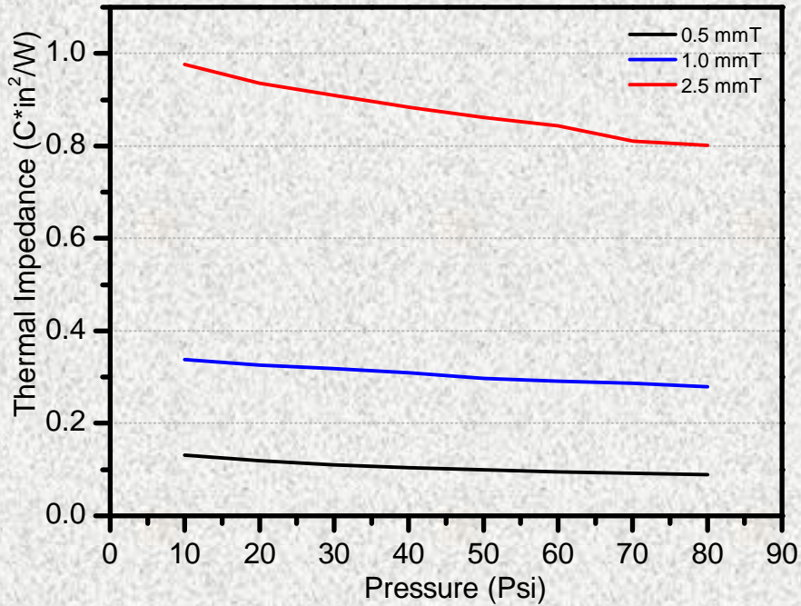
Thermal Impedance of OP-7600 Spec 01
