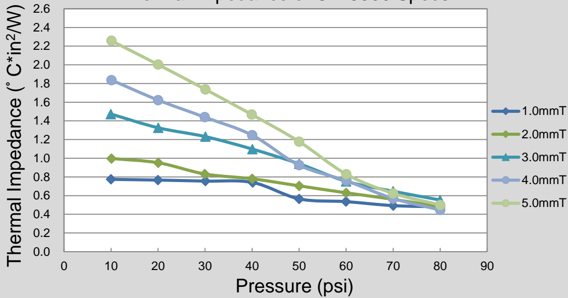
Thermal Impedance of OP-8500 Spec02
